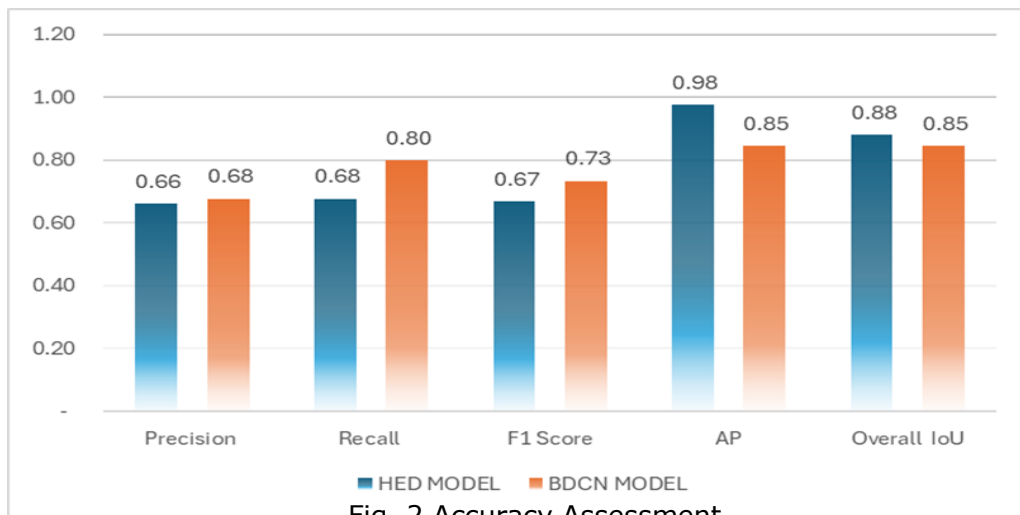
Fig. 2 Accuracy Assessment
